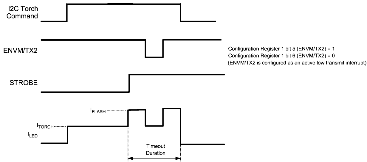
FIGURE 9. ENVM/TX2 Pin is Configured as an Active Low TX Input
