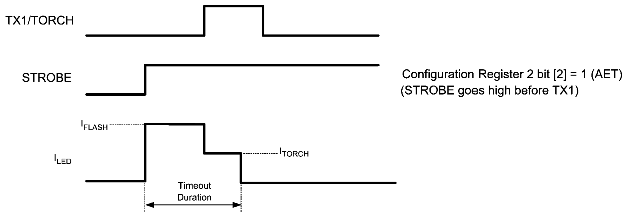
FIGURE 11. Alternative External Torch Mode (STROBE Goes High Before TX1/TORCH, Same as Default with SEM = 0)
