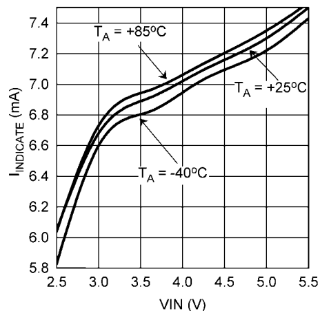
Indicator Current vs V_{IN} , V_{LED1} = 2V (Torch Brightness Register bits[7:6] = 10)
