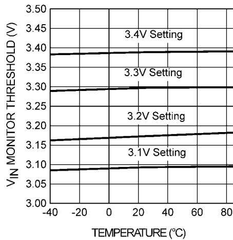
V_{IN} Monitor Thresholds vs Temperature
