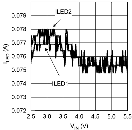
Torch Current vs V_{IN} ( V_{LED1}, V_{LED2} = 3.2V, T_A = +85^\circ C, 75mA setting)
