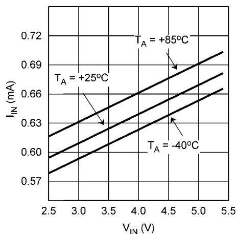
Active (Non-Switching) Supply Current vs V_{IN} ( V_{LED} = 1.5\text{V} )
