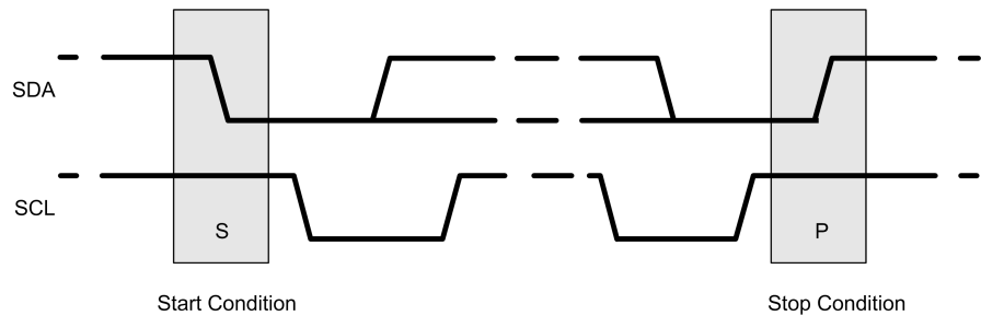
FIGURE 13. Start and Stop Sequences
