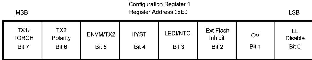
FIGURE 20. Configuration Register1 Description
