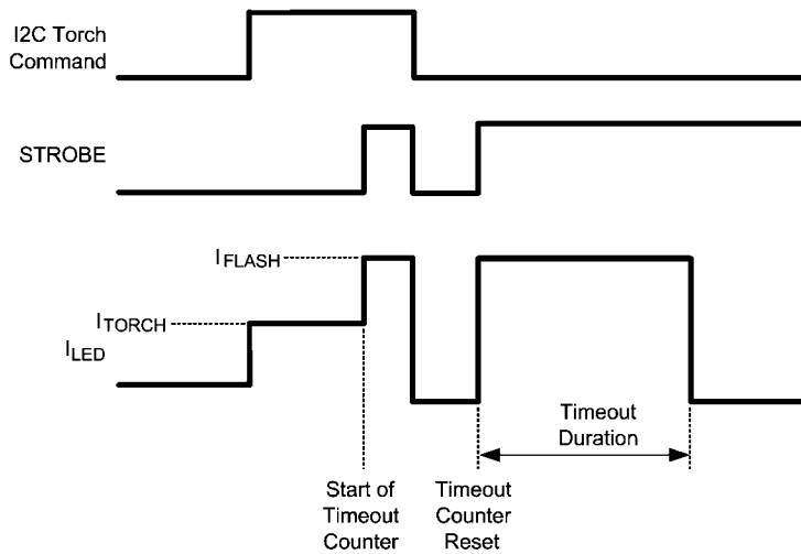
FIGURE 6. STROBE Input is Level Sensitive (Default State, STR bit = 0)
