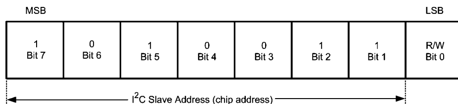
FIGURE 15. Device Address
