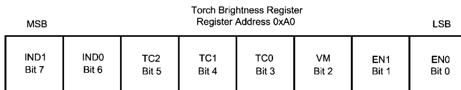
FIGURE 16. Torch Brightness Register Description
