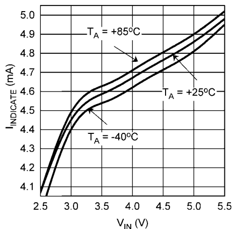
Indicator Current vs V_{IN} , V_{LED1} = 2V (Torch Brightness Register bits[7:6] = 01)
