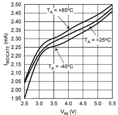
Indicator Current vs V_{IN} , V_{LED1} = 2\text{V} (Torch Brightness Register bits [7:6] = 00)
