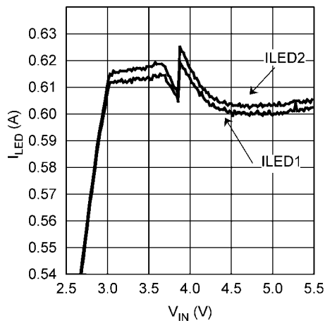
Flash Current vs V_{IN} ( V_{LED1}, V_{LED2} = 3.2V, T_A = +85^\circ C, 600mA setting)
