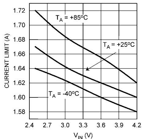
Closed Loop Current Limit vs V_{IN} (Flash Duration Register bits [6:5] = 01, (Note 8))
