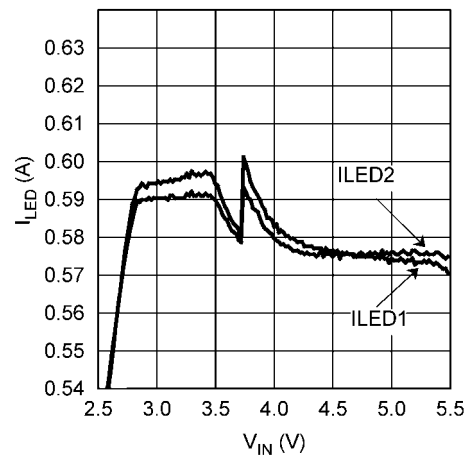
Flash Current vs V_{IN} ( V_{LED1}, V_{LED2} = 3.2V, T_A = -40^\circ C, 600mA setting)
