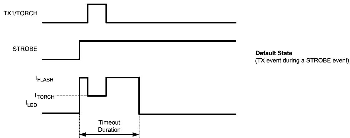
FIGURE 4. TX1 Event During a Flash Event (Default State, TX1/TORCH is an Active High TX Input)
