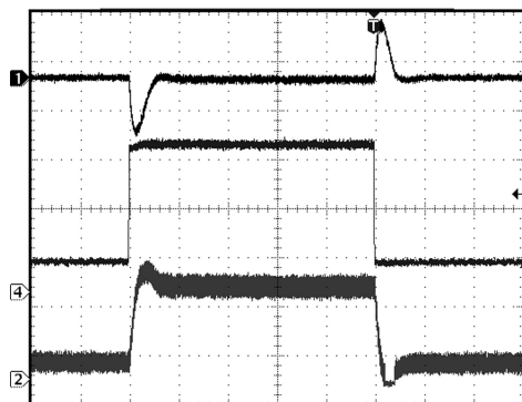
Load Transient V_{IN} = 3.6V (Voltage Output Mode, V_{OUT} = 5V )
