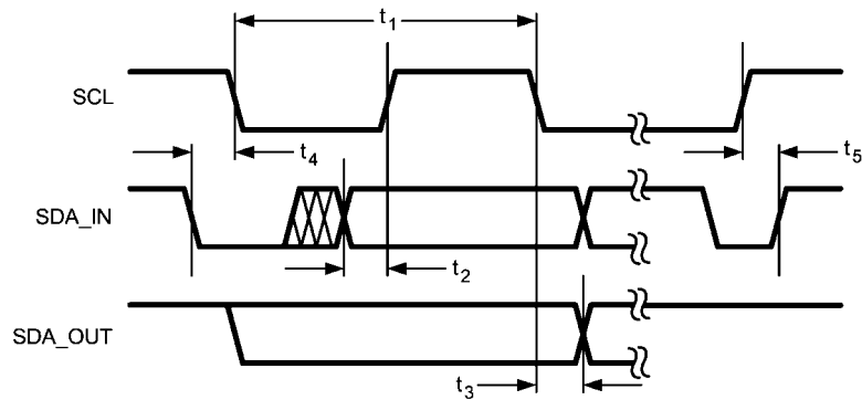
FIGURE 14. I 2 C-Compatible Timing
