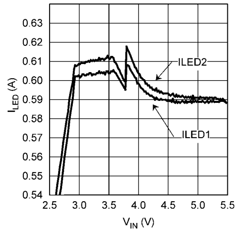
Flash Current vs V_{IN} ( V_{LED1}, V_{LED2} = 3.2V, T_A = +25^\circ C, 600mA setting)
