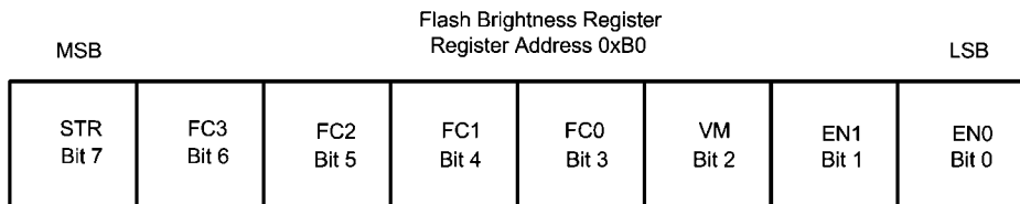
FIGURE 17. Flash Brightness Register Description
