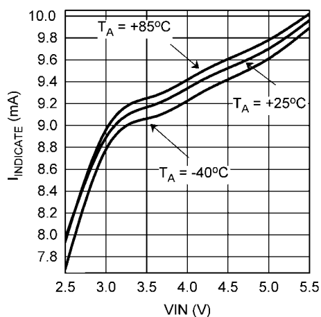
Indicator Current vs V_{IN} , V_{LED1} = 2V (Torch Brightness Register bits[7:6] = 11)
