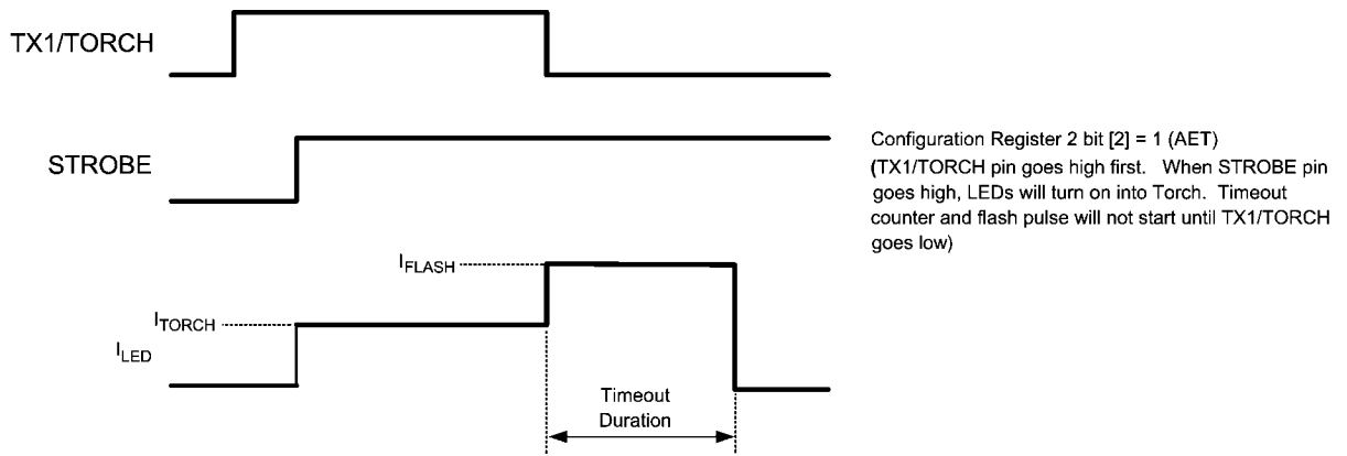
FIGURE 10. Alternative External Torch Mode (TX1/TORCH Turns on Before STROBE)
