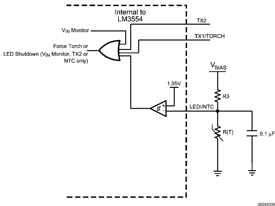
FIGURE 25. Thermistor Voltage Divider and Sensing Circuit
