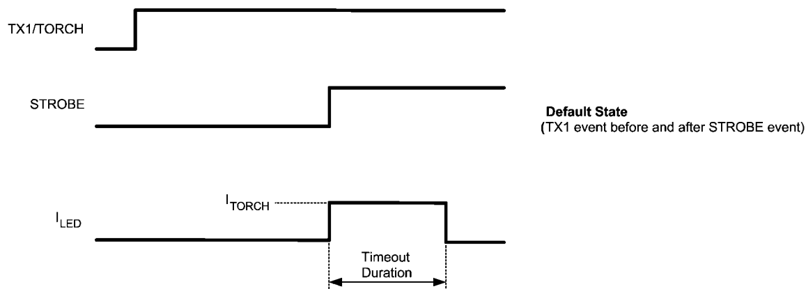
FIGURE 5. TX1 Event Before and After Flash Event (Default State, TX1/TORCH is an Active High TX Input)
