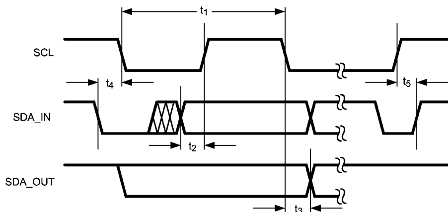
FIGURE 1. I²C Timing
