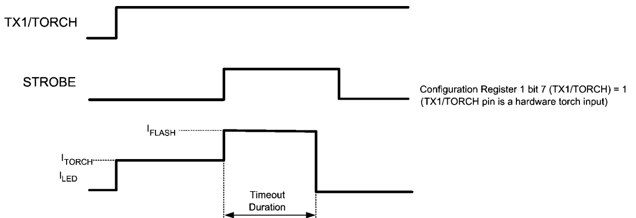
FIGURE 12. TX1/TORCH Configured as a Hardware Torch input
