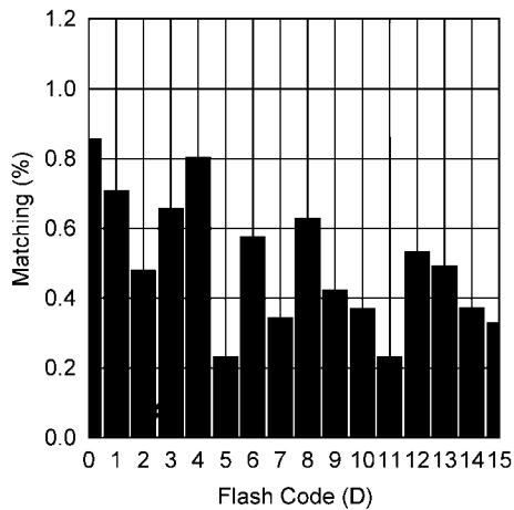
Flash Current Matching vs Code ( V_{IN} = 3.6V, V_{LED1}, V_{LED2} = 3.2V, T_A = -40^\circ C to +85^\circ C , (Note 10))
