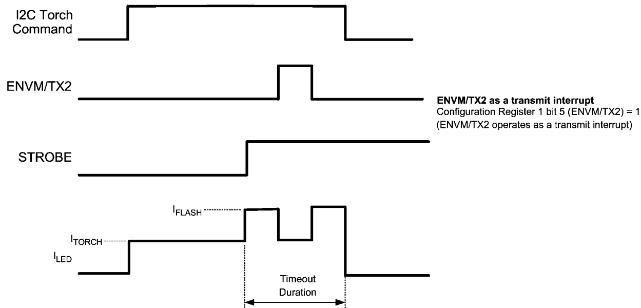
FIGURE 8. ENVM/TX2 Pin is Configured as an Active High TX Input
