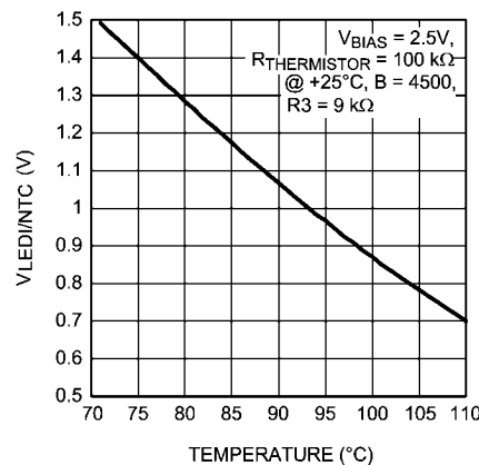
FIGURE 24. Thermistor Resistive Divider Response vs Temperature
