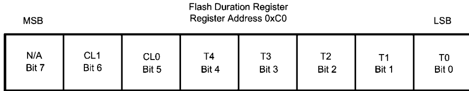
FIGURE 18. Flash Duration Register Description
