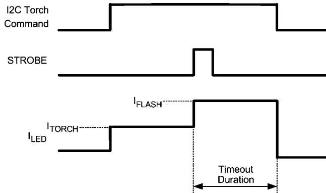
FIGURE 7. STROBE Input is Edge Sensitive (STR bit = 1)
