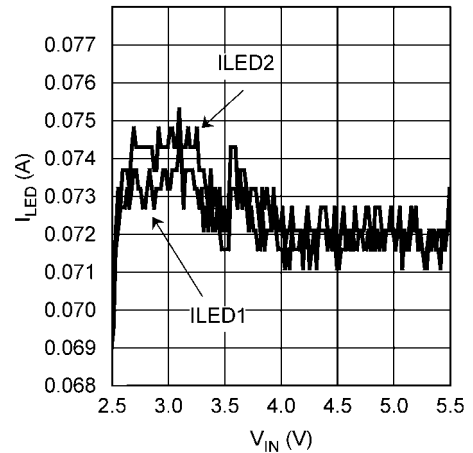
Torch Current vs V_{IN} ( V_{LED1}, V_{LED2} = 3.2V, T_A = -40^\circ C, 75mA setting)
