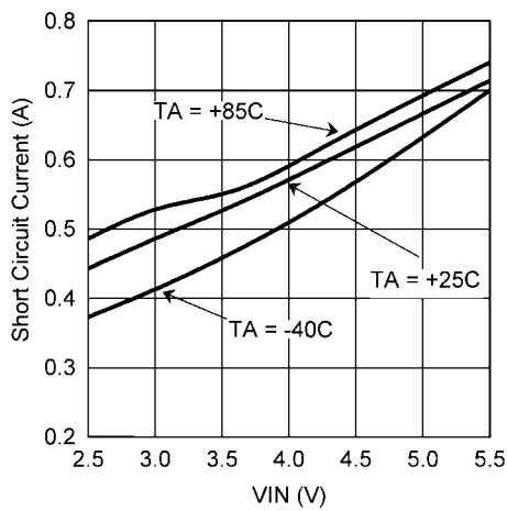
Short Circuit Current Limit vs V_{IN}
