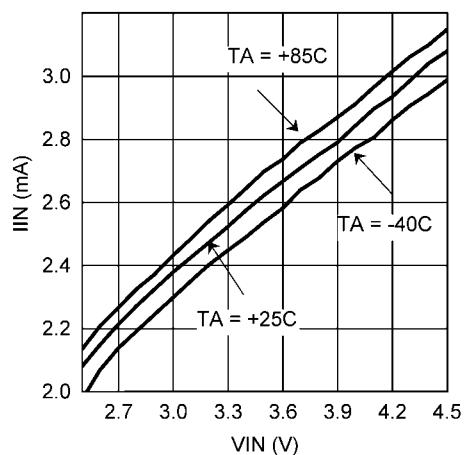
Active (Switching) Supply Current vs V_{IN} ( V_{OUT} = 5\text{V} , I_{OUT} = 400\text{mA} )
