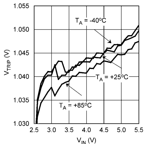
NTC Comparator Trip Threshold vs V_{IN}
