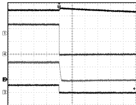
Flash Pulse to HWEN Low Single LED, I_{LED} = 1.2A
