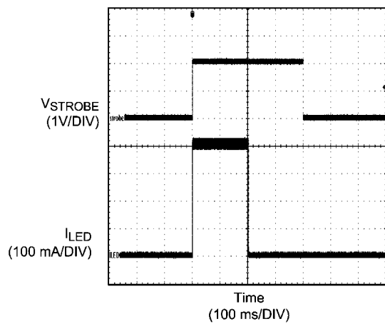
Level Sensitive Strobe with Timeout
