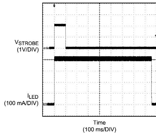
Level Sensitive Strobe without Timeout
