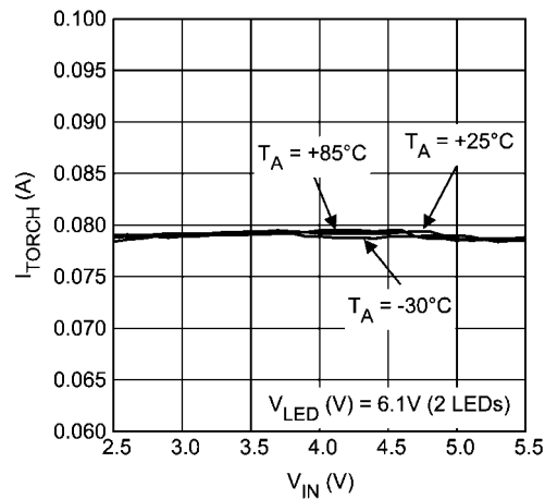
80mA Torch Current vs Input Voltage 2 LED
