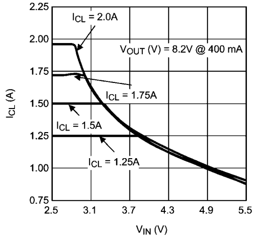
Inductor Current Limit vs Input Voltage
