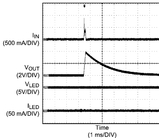
VLED Short to GND Fault
