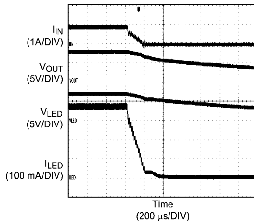
Ramp-Down 2 LEDs Simple Mode
