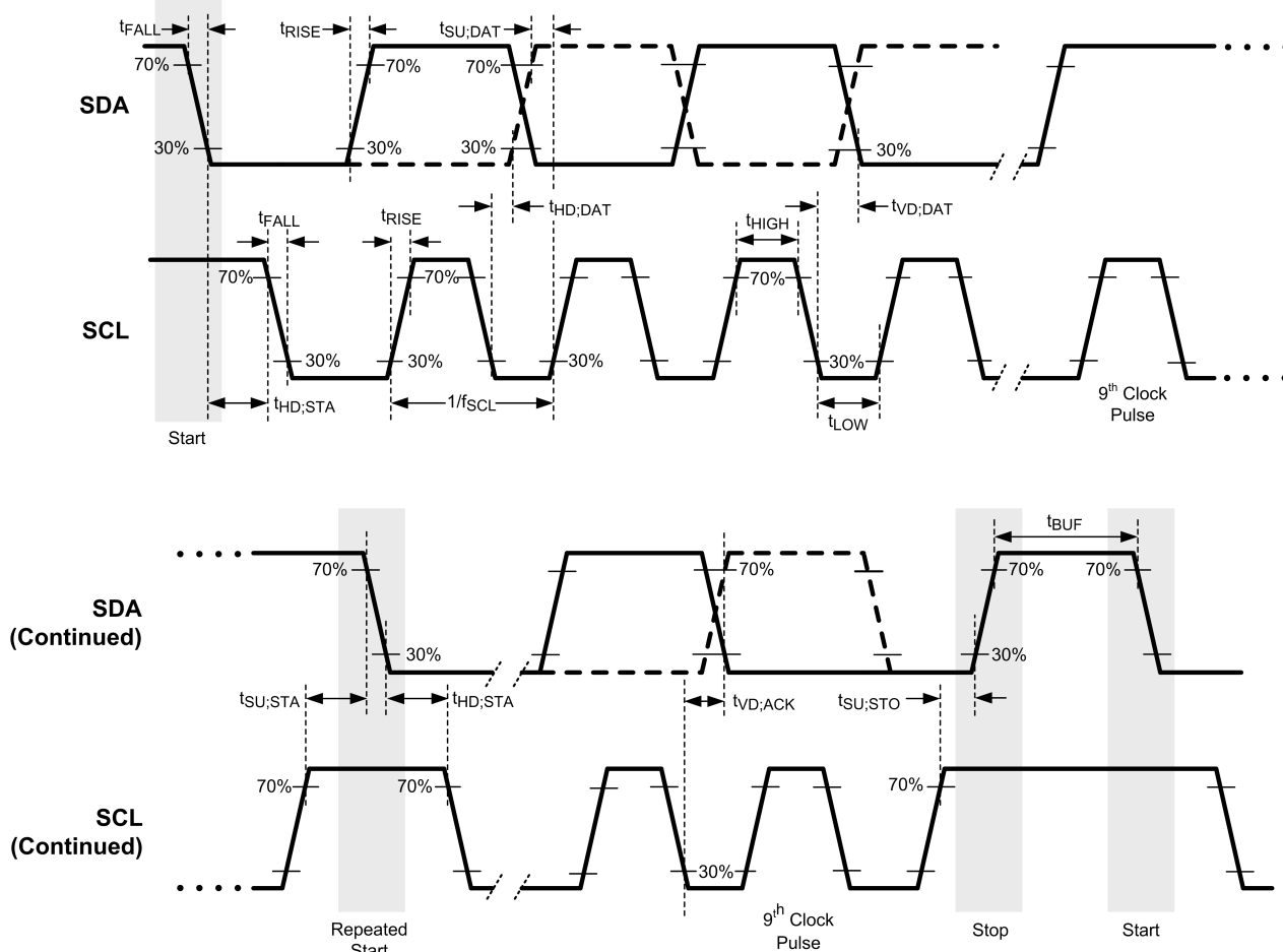
FIGURE 13. I²C-Compatible Timing
