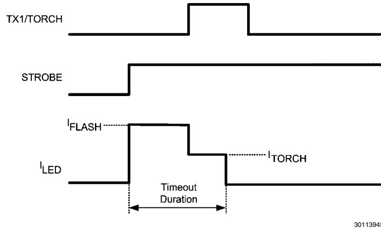
FIGURE 10. Alternative External Torch Mode (STROBE Goes High Before TX1/TORCH, Same as Normal TX1 Operation)
