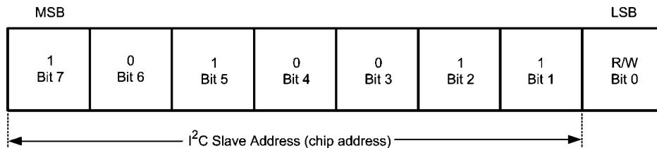
FIGURE 14. Device Address
