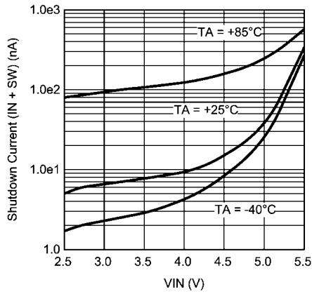
Shutdown Current vs V_{IN} ( V_{HWEN} = GND )
