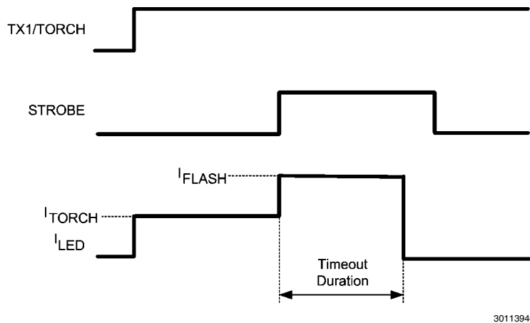
FIGURE 11. TX1/TORCH Pin is Configured as a Hardware Torch Input
