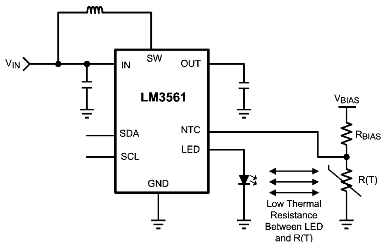
FIGURE 15. NTC Circuit
