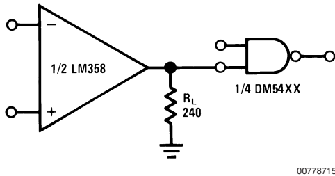
Driving TTL
