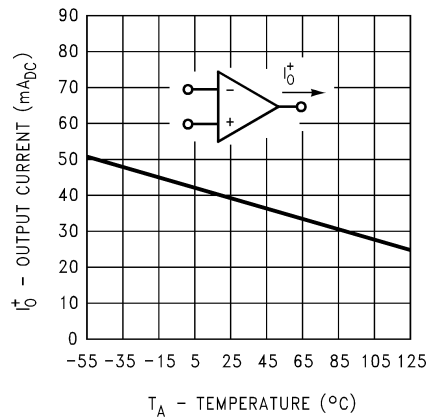
Current Limiting
