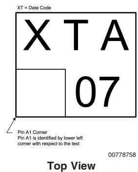
LM358TP micro SMD Marking Orientation
