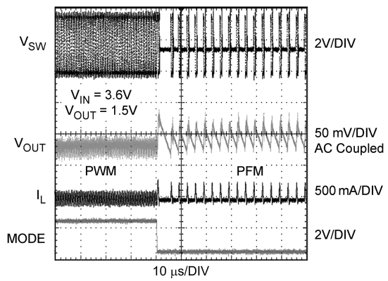
Mode Change by Mode Pin V_{OUT} = 1.5V (PWM to PFM)
