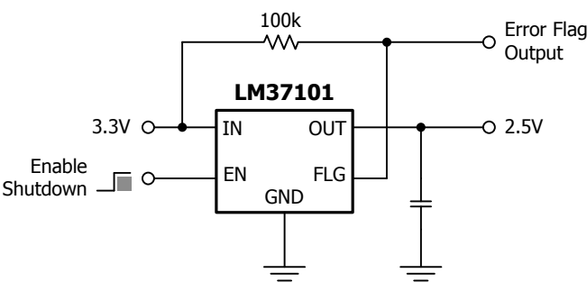
2.5V / 1A Regulator with Error Flag
