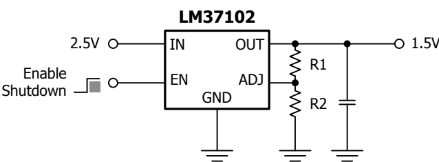
1.5V / 1A Adjustable Regulator
