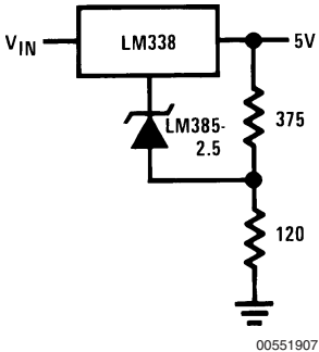
Improving Regulation of Adjustable Regulators
