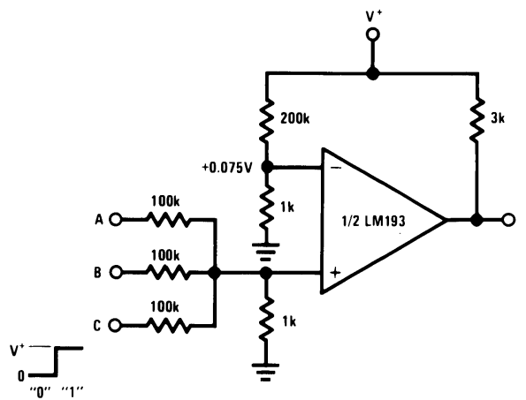
Figure 29. OR Gate
