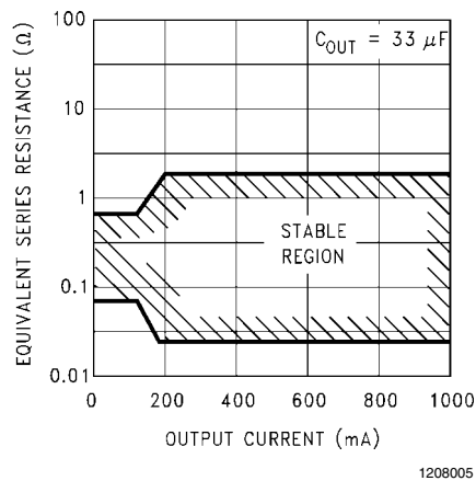
FIGURE 1. ESR Limits
