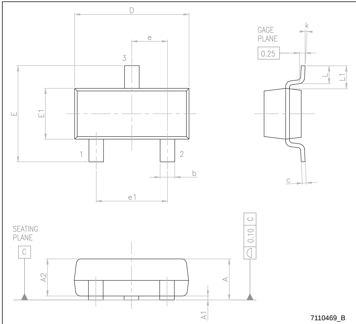
Figure 9. SOT23-3L dimensions
