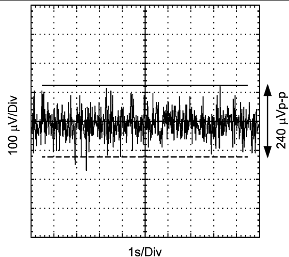
Figure 26. 0.1–10 Hz Noise
