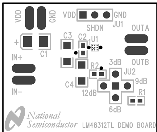
Top Silkscreen
