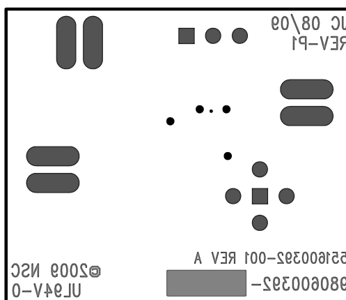
Bottom Silkscreen
