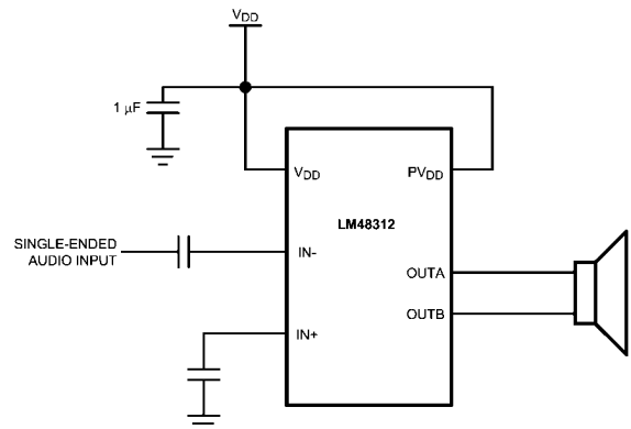
FIGURE 4. Single-Ended Input Configuration
