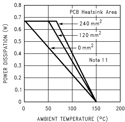
Power Derating - 8 Bump \mu\text{SMD} P_{D\text{MAX}} = 670\text{mW} V_{DD} = 5V, R_L = 8\Omega
