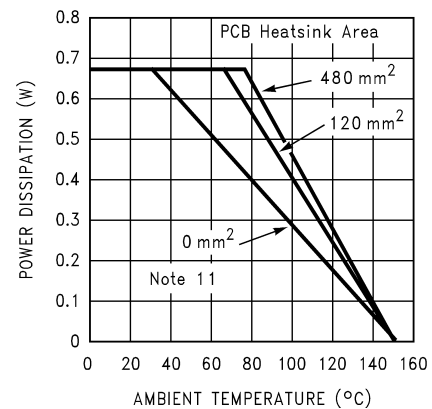
Power Derating - 9 Bump \mu\text{SMD} P_{D\text{MAX}} = 670\text{mW} V_{DD} = 5V, R_L = 8\Omega
