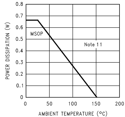
Power Derating - MSOP P_{D\text{MAX}} = 670\text{mW} V_{DD} = 5V, R_L = 8\Omega
