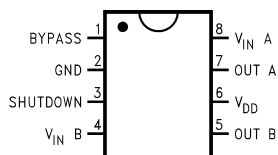
Figure 2. VSSOP Package Top View See Package Number DKG0008A
