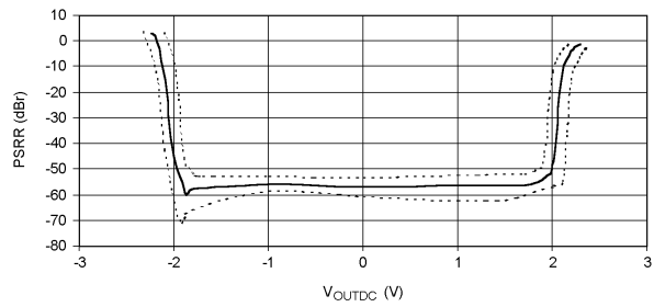
PSRR vs DC Output Voltage
