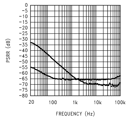
LM4890 vs LM4877 Power Supply Rejection Ratio V_{DD} = 3V , Input Grounded = 10Ω Output Load = 8Ω, 200mV Ripple
