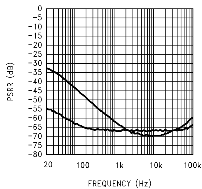
LM4890 vs LM4877 Power Supply Rejection Ratio V_{DD} = 5V , Input Grounded = 10Ω Output Load = 8Ω, 200mV Ripple
