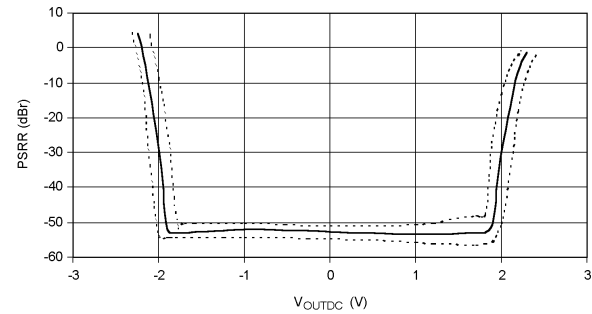
PSRR vs DC Output Voltage
