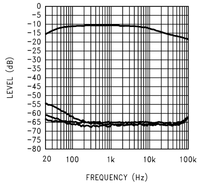
Power Supply Rejection Ratio vs Bypass Capacitor Size V_{DD} = 5V , Input Grounded = 10Ω, Output Load = 8Ω
