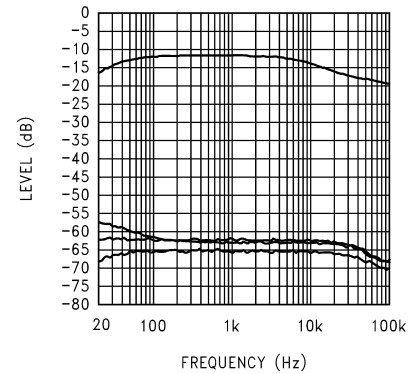
Power Supply Rejection Ratio vs Bypass Capacitor Size V_{DD} = 3V , Input Grounded = 10Ω, Output Load = 8Ω
