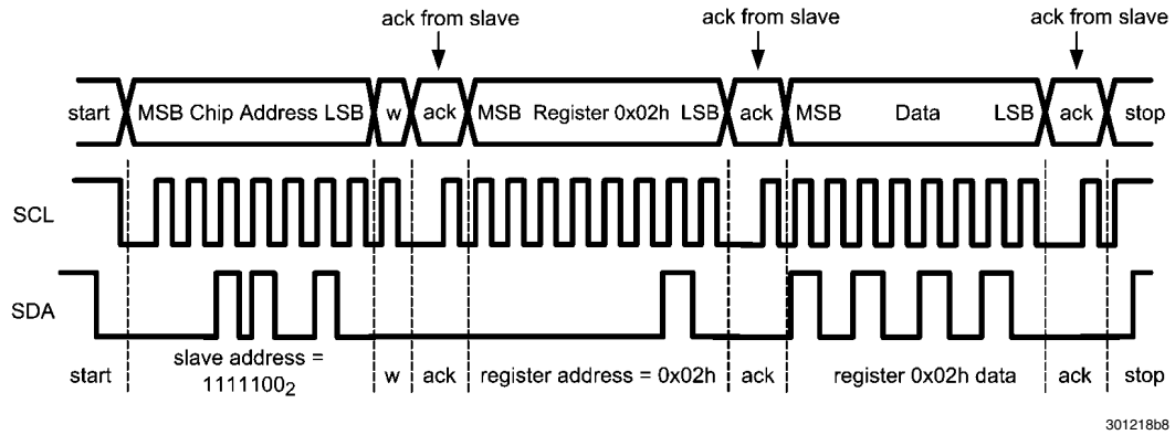
FIGURE 6. Example I 2 C Write Cycle
