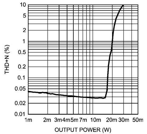
THD+N vs Output Power R_L = 16\Omega, f = 1kHz, \text{Mode 6}
