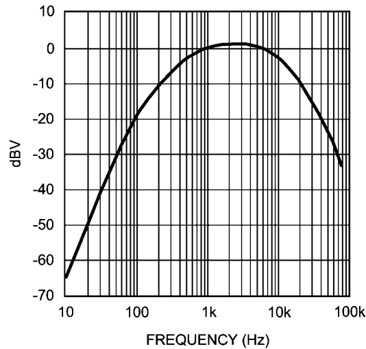
FIGURE 15. A-Weighted Filter
