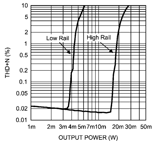
FIGURE 9. Class G Disabled (Low/High Supply Rails)
