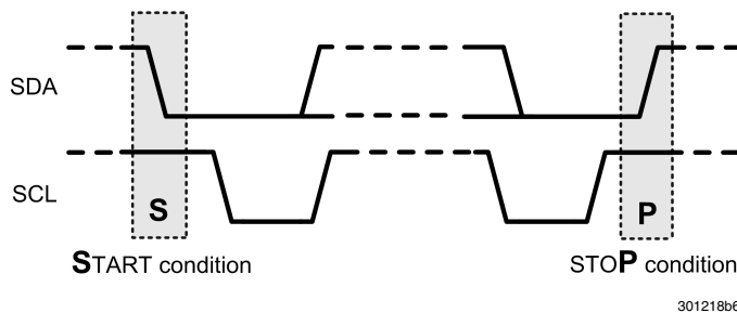
FIGURE 4. I 2 C Start and Stop Conditions
