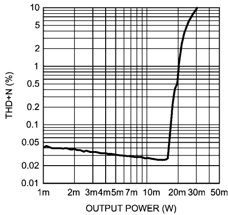
THD+N vs Output Power R_L = 16\Omega, f = 1kHz, \text{Mode 4}
