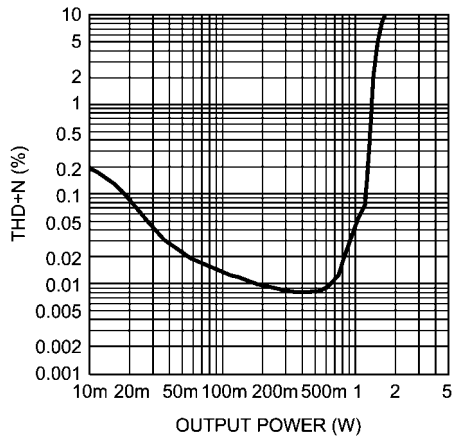
THD+N vs Output Power V_{DD} = 5V, R_L = 15\mu H + 8\Omega + 15\mu H f = 1kHz, \text{Mode 3}
