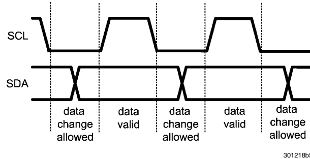
FIGURE 3. I 2 C Signals: Data Validity
