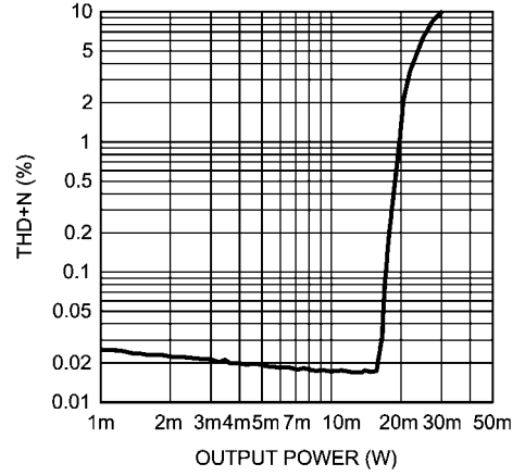
THD+N vs Output Power R_L = 32\Omega, f = 1kHz, \text{Mode 4}
