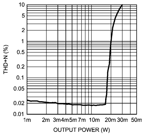
THD+N vs Output Power R_L = 32\Omega, f = 1kHz, \text{Mode 6}
