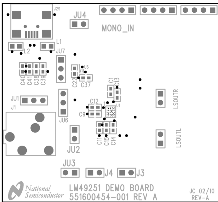
Top Silkscreen
