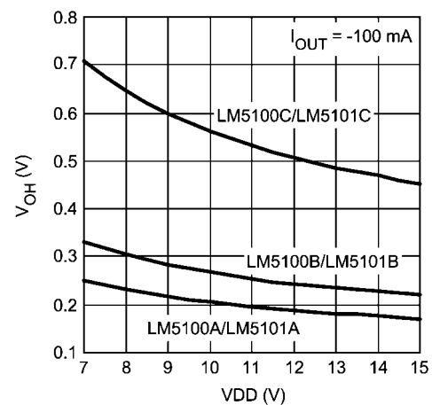
LO &amp; HO Gate Drive - Output High Voltage vs VDD
