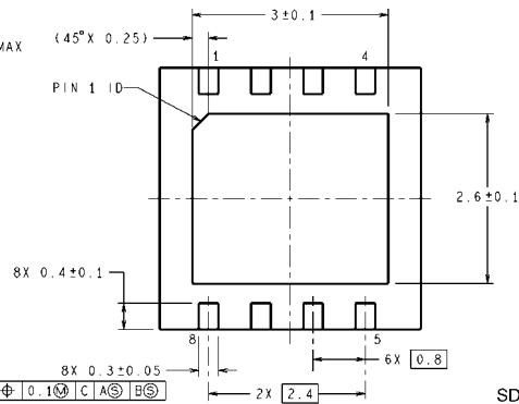
LLP-8 Outline Drawing NS Package Number SDC08A
