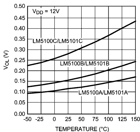
LO &amp; HO Gate Drive - Low Level Output Voltage vs Temperature
