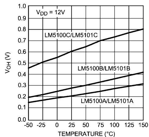
LO &amp; HO Gate Drive - High Level Output Voltage vs Temperature
