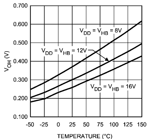
LO &amp; HO Gate Drive—High Level Output Voltage vs Temperature
