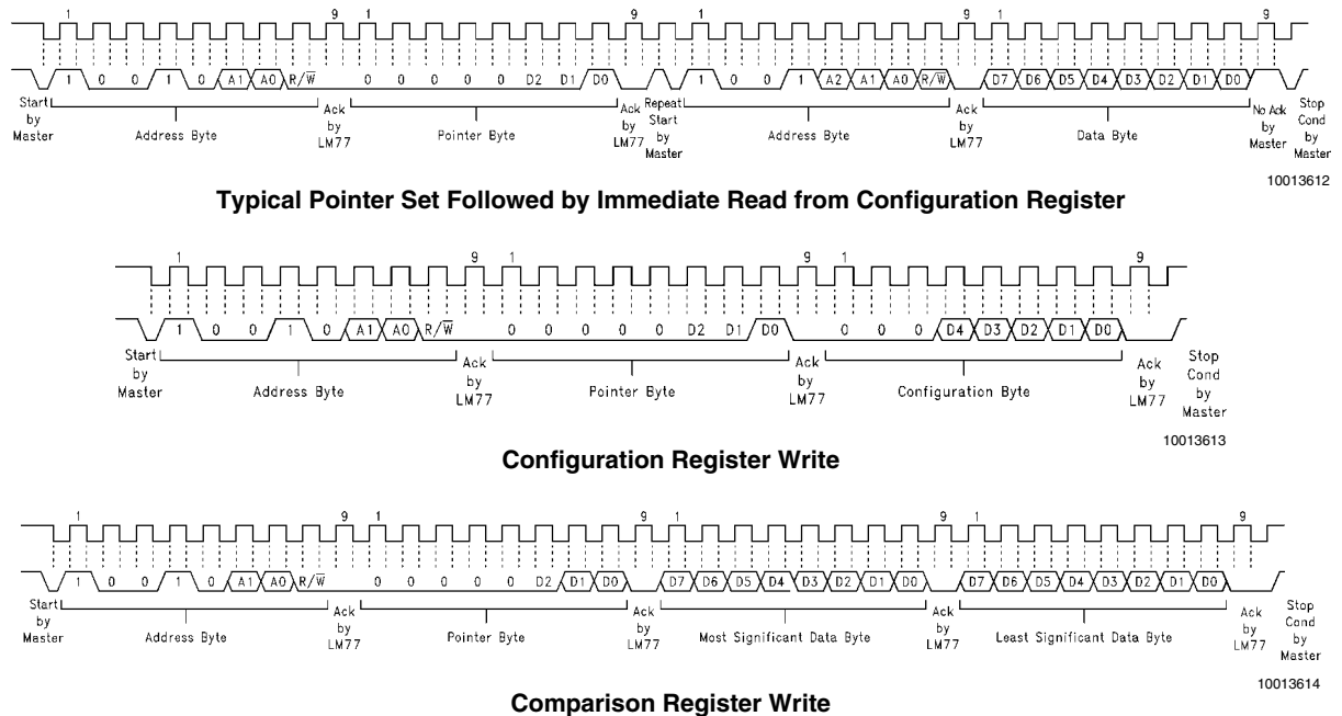
FIGURE 6. Timing Diagrams
