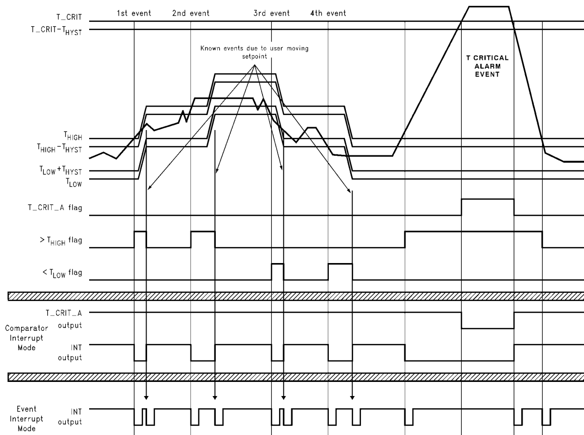
FIGURE 7. Temperature Response Diagram for ACPI Implementation
