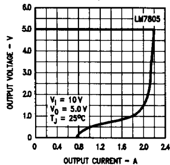
Current-Limiting Characteristics
