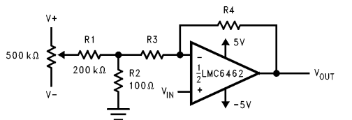
FIGURE 9. Inverting Configuration Offset Voltage Adjustment
