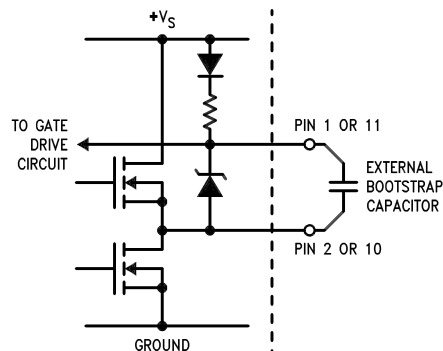
FIGURE 5. Bootstrap Circuitry
