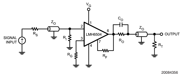
FIGURE 5. TRANSMISSION LINE MATCHING
