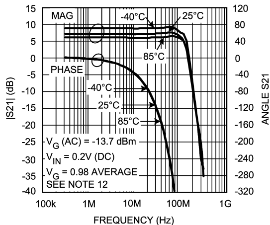
Gain Control Frequency Response
