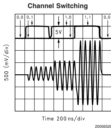
FIGURE 7. PGA Output
