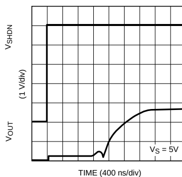
Figure 46. Turn-on Time
