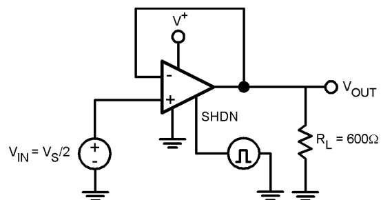
FIGURE 6. Turn-off Time
