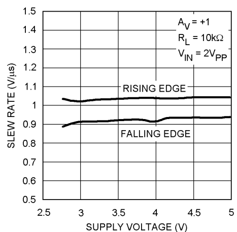
Slew Rate vs. V_{SUPPLY}
