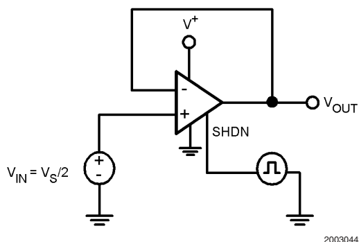
FIGURE 5. Turn-on Time
