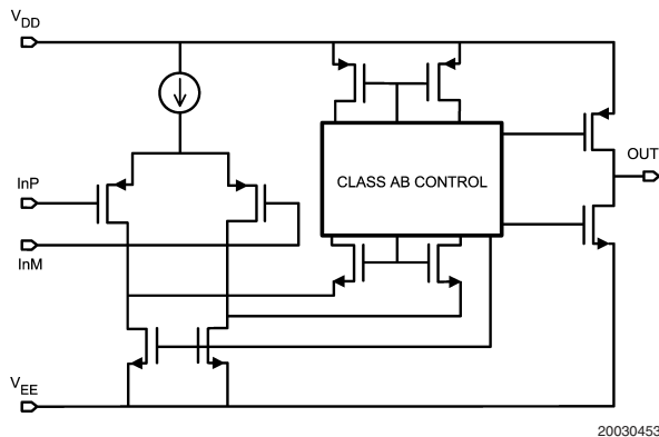
FIGURE 1. Simplified Schematic
