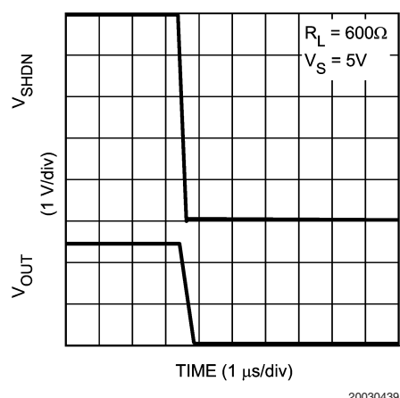
FIGURE 4. Turn-off Time
