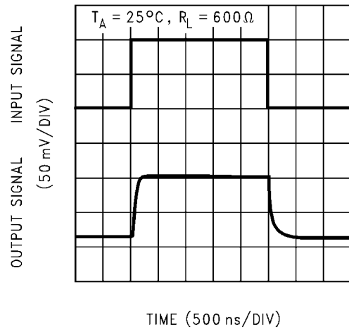
Non-Inverting Small Signal Pulse Response
