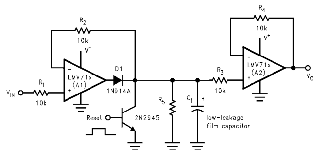
FIGURE 7. Peak Detector
