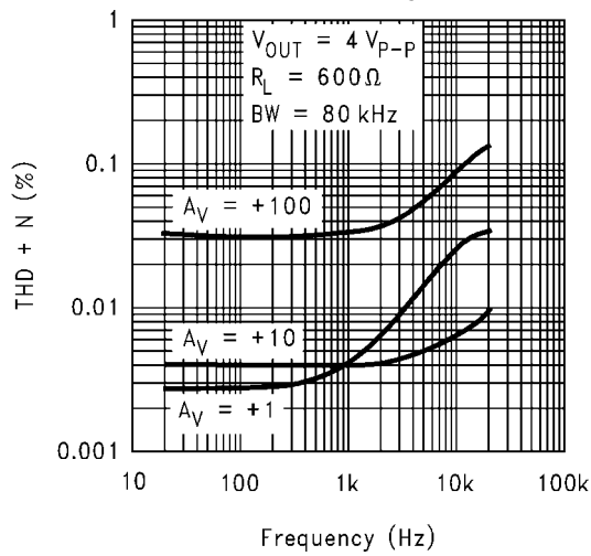
THD+N vs. Frequency ( V_S = 5V )
