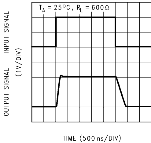
Non-Inverting Large Signal Pulse Response
