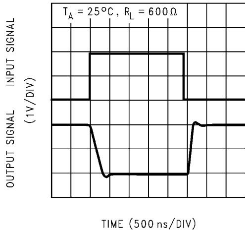
Inverting Large Signal Pulse Response
