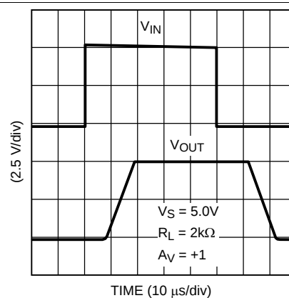
Figure 22. Large Signal Noninverting Response
