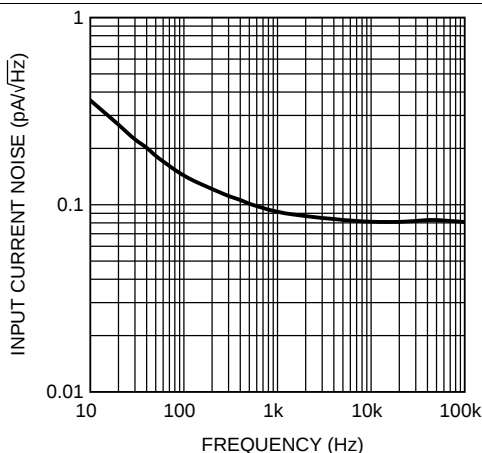
Figure 13. Input Current Noise vs. Frequency
