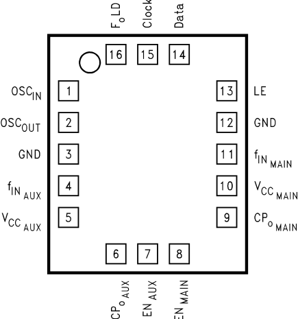
10012922 Order Number LMX1600SLB, LMX1601SLB, or LMX1602SLB NS Package Number SLB16A
