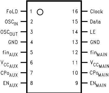
10012902 Order Number LMX1600TM, LMX1601TM, or LMX1602TM NS Package Number MTC16
