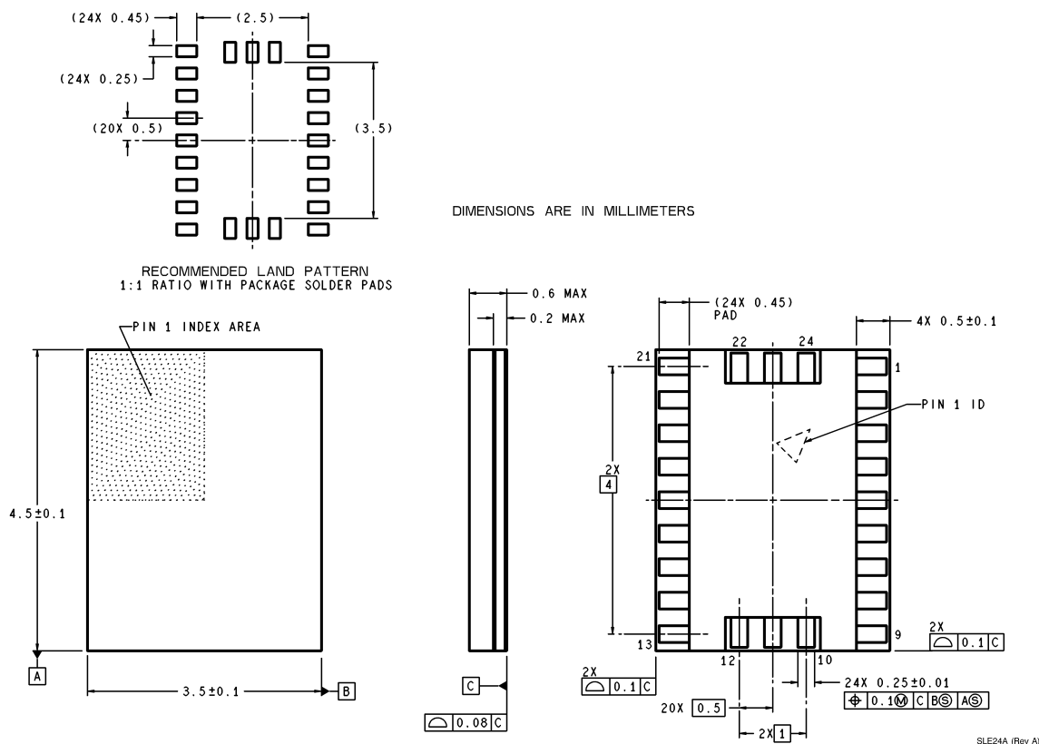
Ultra Thin Chip Scale Package (SLE) For Tape and Reel (2500 Units per Reel) Order Number LMX2364SLEX NS Package Number SLE24A
