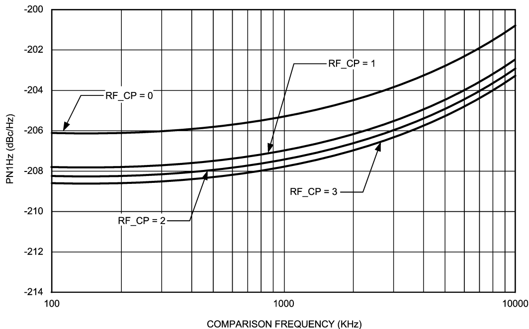
RF PLL 1 Hz Normalized Phase Noise (Fractional Mode)
