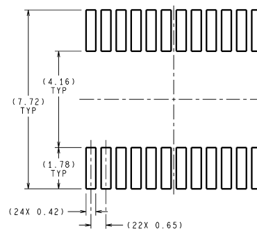
LAND PATTERN RECOMENDATION
