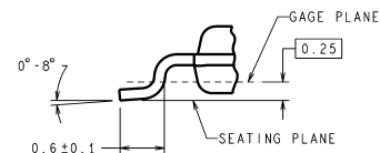
DETAIL A TYPICAL
