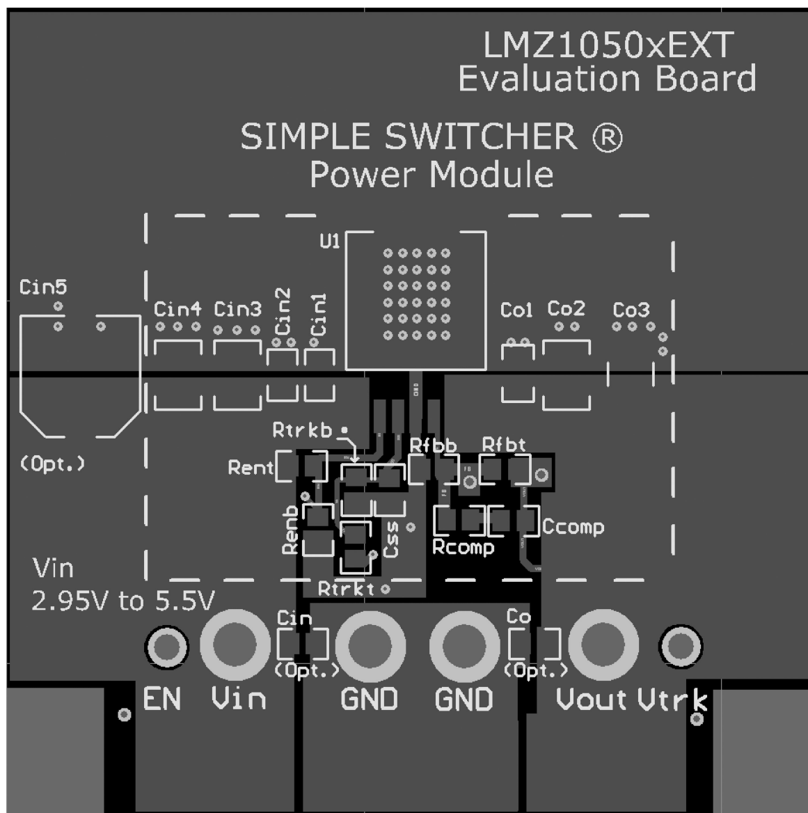
FIGURE 6. Top Copper
