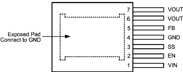
Top View 7-Lead TO-PMOD
