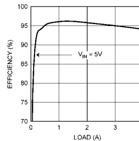
Efficiency ( V_{OUT} = 3.3\text{V} )
