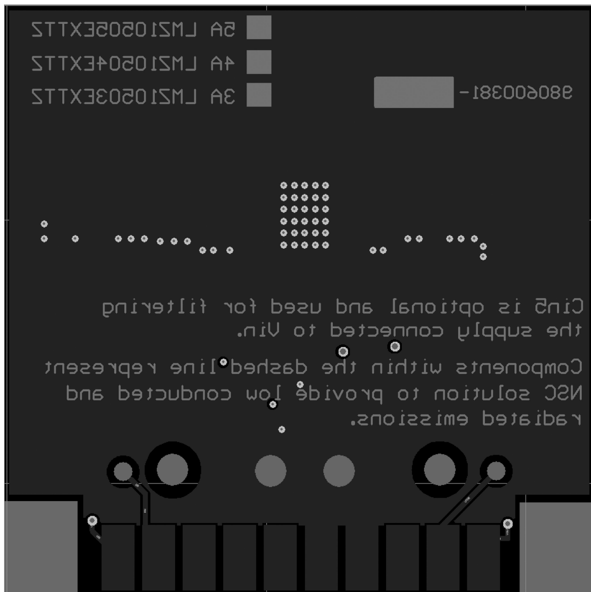
FIGURE 9. Bottom Copper
