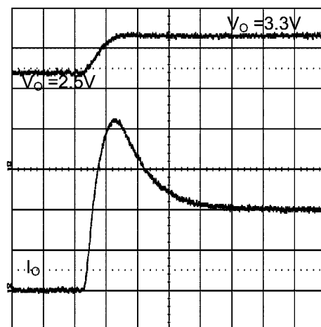
Pre-Biased Startup
