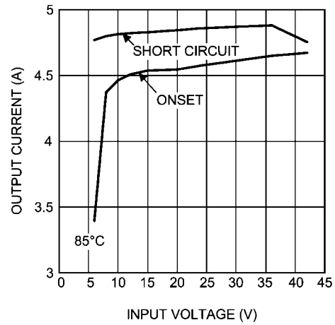
Current Limit 3.3V_{OUT} @ 85^{\circ}C
