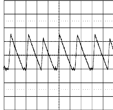
Transition Mode Operation V_{IN} = 24V, V_O = 3.3V, I_O = 0.5A \text{ } 2 \mu\text{sec/div}
