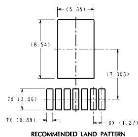
7-Lead TZA Package NS Package Number TZA07A
