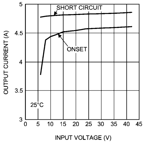
Current Limit 3.3V_{OUT} @ 25^{\circ}C
