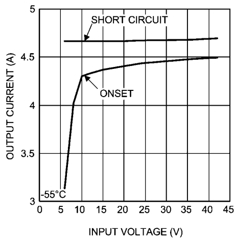
Current Limit 3.3V_{OUT} @ -55^{\circ}C
