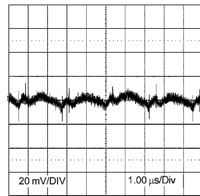
Output Ripple 24V IN 3.3V O 3A, BW = 200 MHz
