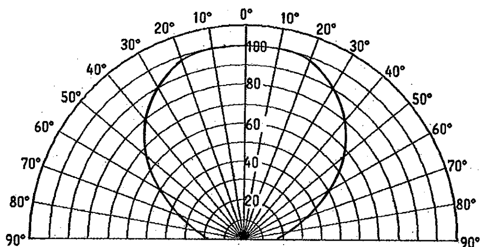
指向特性 Directive Characteristics
