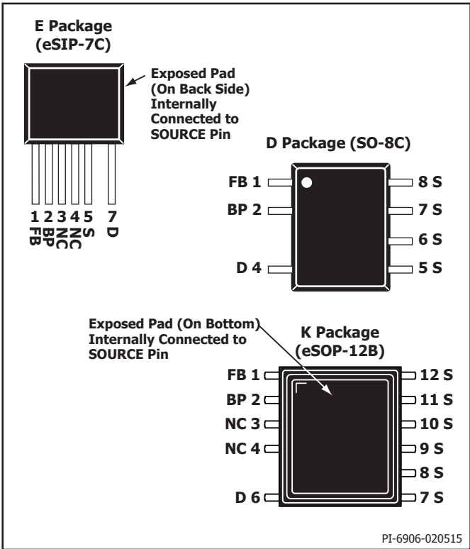
Figure 3. Pin Configuration.
