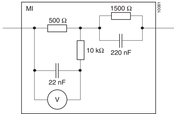
Fig. 11 Measuring instrument (MI) for earth leakage current tests according to IEC/EN 60950.
