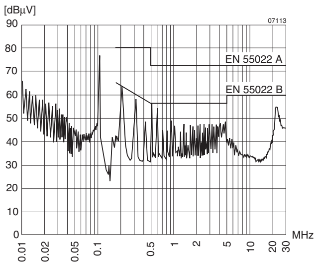
Fig. 8 Typical conducted disturbances (quasi-peak) at the input measured according to EN 55011/55022 at V_{i\text{ nom}} and I_{o\text{ nom}} . LOK4601-2R, V_i = 230 VAC.
