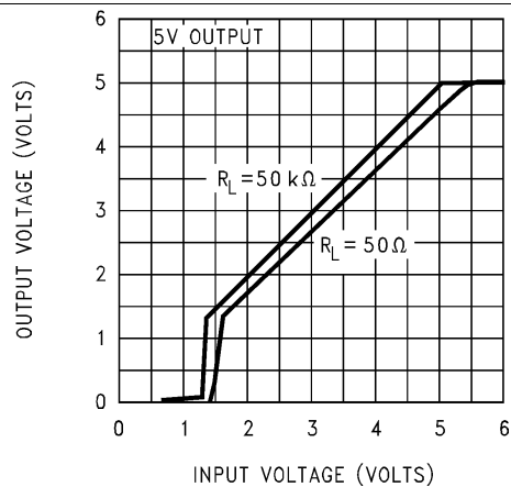
Figure 2. Dropout Characteristics
