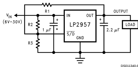
FIGURE 3. Snap-On/Snap-Off Output
