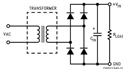
FIGURE 5. Transformer Powered Input Supply
