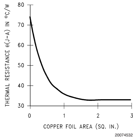
FIGURE 1. \theta_{\text{JA}} vs Copper (1 Ounce) Area for TO-263 package
