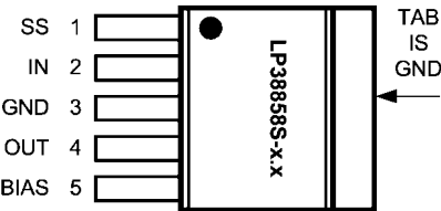
TO263-5, Top View
