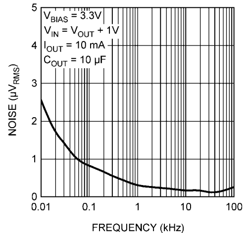
Output Noise
