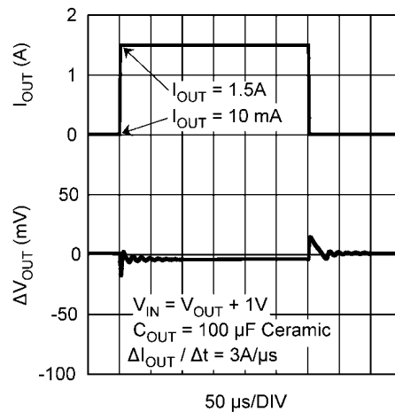
Load Transient Response, C OUT = 100 \mu F Ceramic
