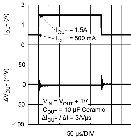
Load Transient Response, C OUT = 10 \mu F Ceramic
