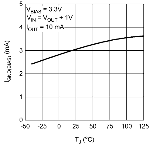
V_{BIAS} Ground Pin Current ( I_{GND(BIAS)} ) vs Temperature
