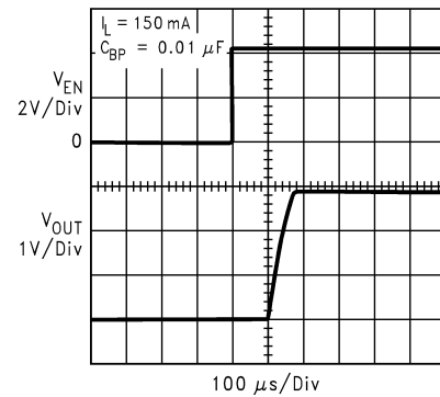
Enable Response ( V_{IN} = 4.2\text{V} )
