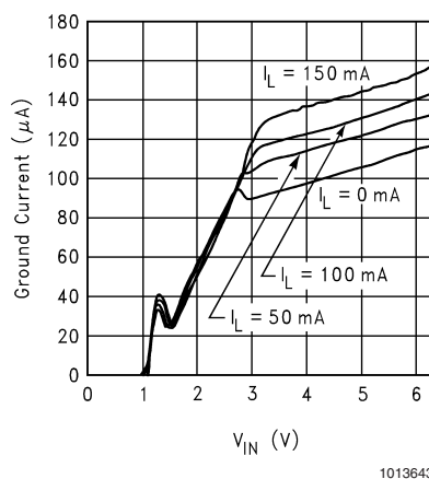
Ground Current vs V_{IN} @ 25^\circ C
