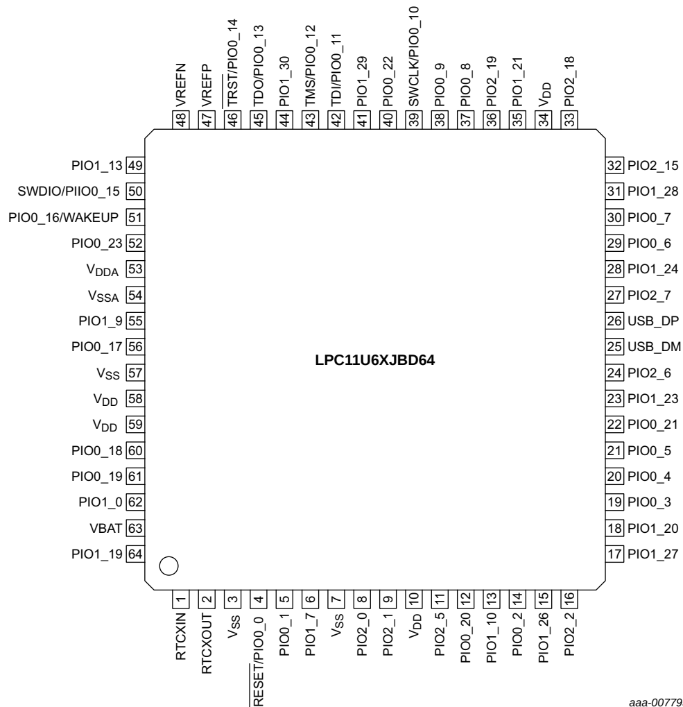
Fig 5. LQFP64 pinning
