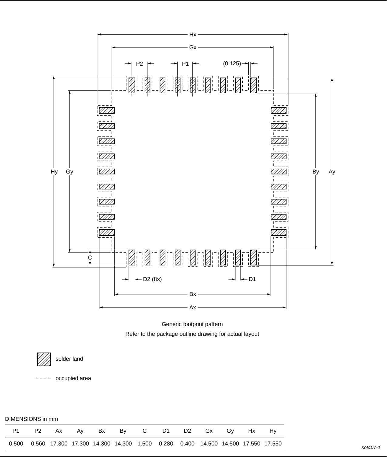
Fig 50. Reflow soldering for the LQFP100 package
