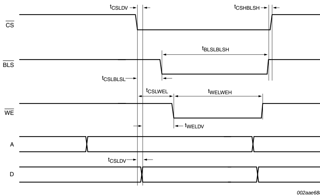
Fig 28. External memory write access
