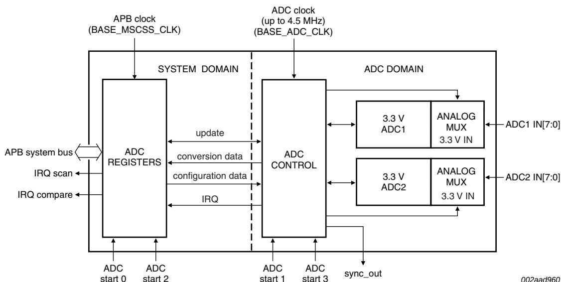
Fig 9. ADC block diagram
