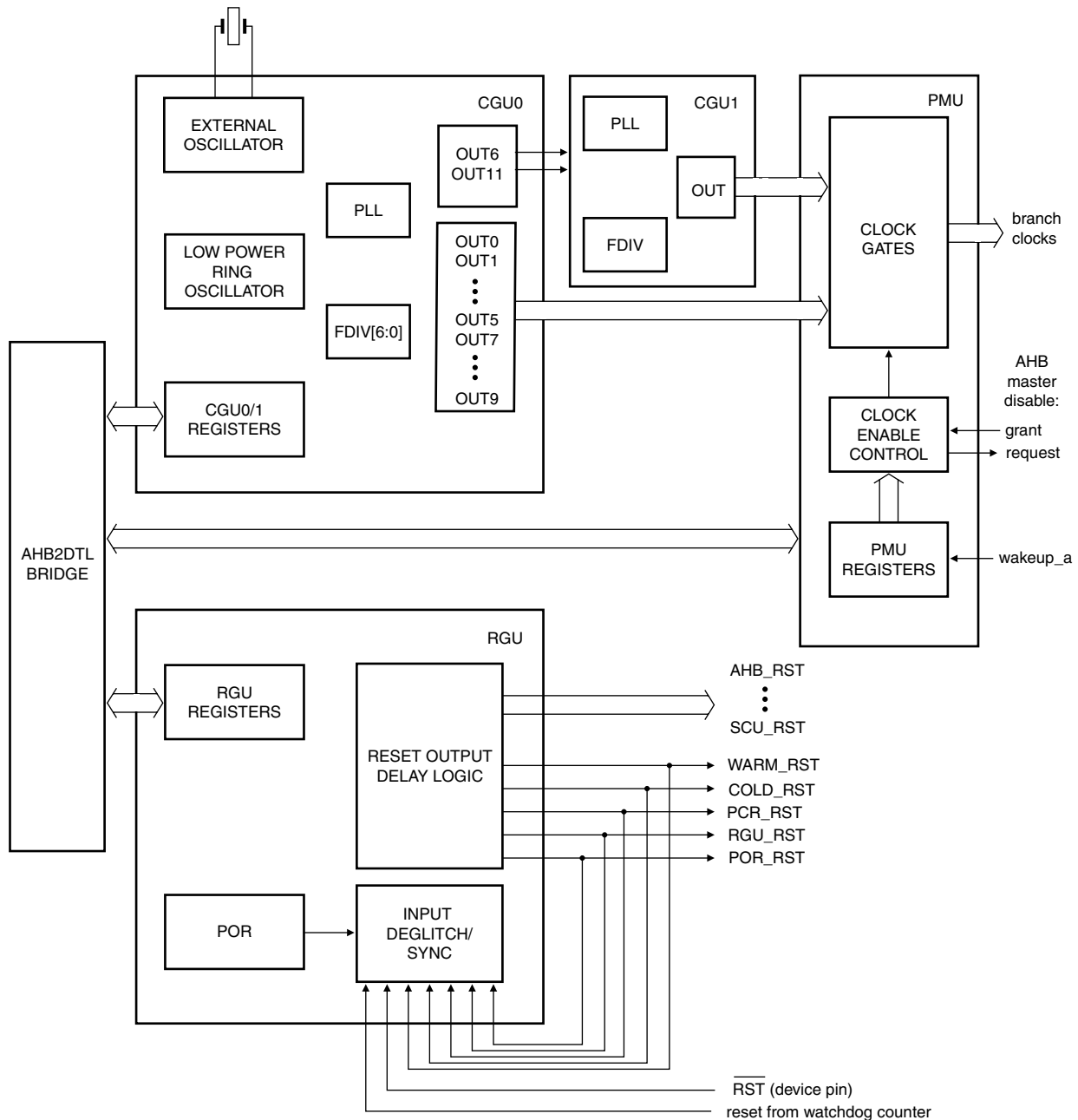
Fig 11. Power, Clock, and Reset control Sub System (PCRSS) block diagram
