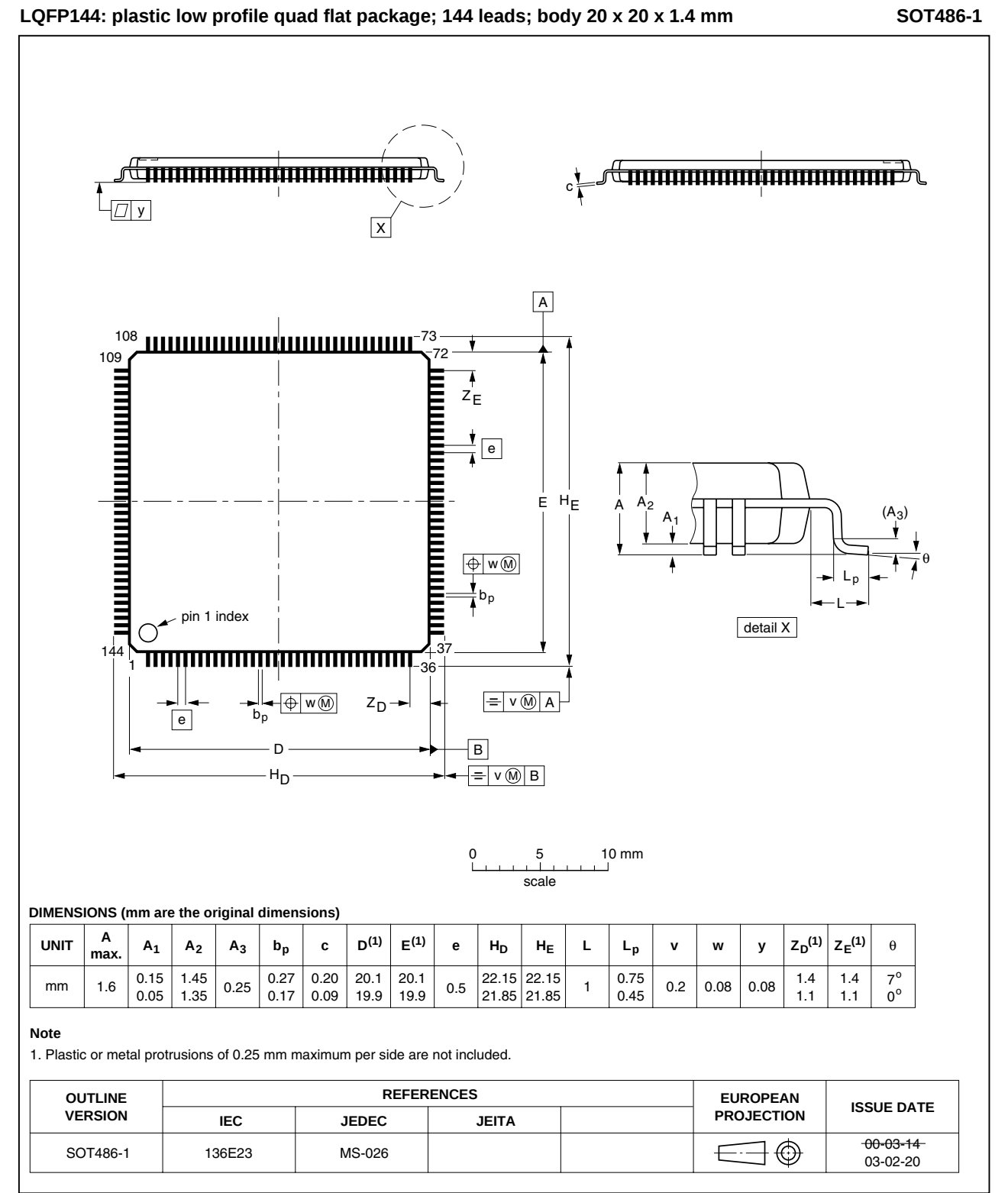
Fig 34. Package outline SOT486-1 (LQFP144)
