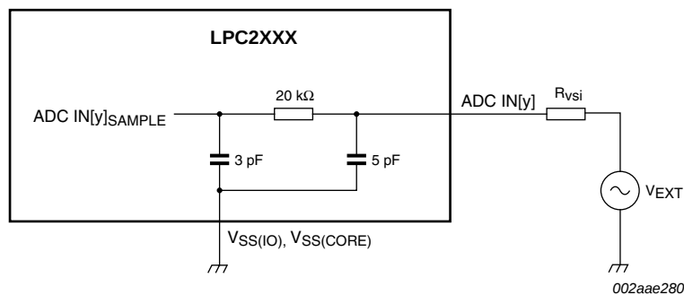
Fig 16. Suggested ADC interface - LPC2917/2919/01 ADC1/2 IN[y] pin
