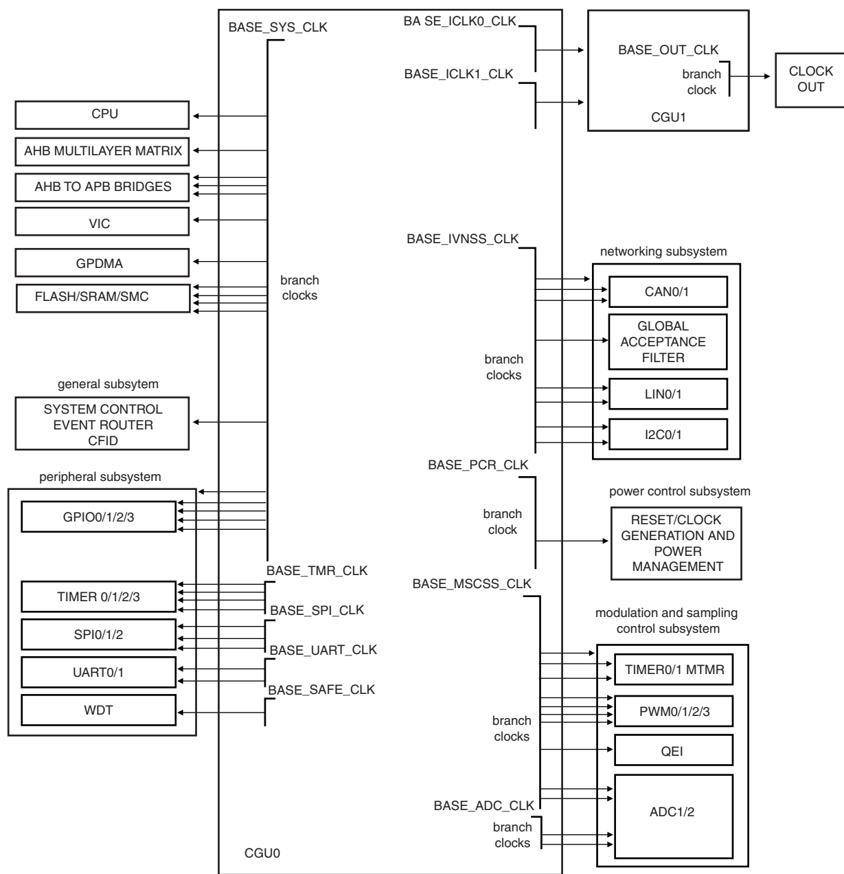
Fig 4. LPC2917/2919/01 block diagram, overview of clock areas
