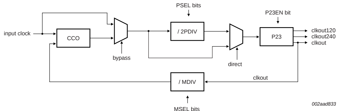
Fig 14. PLL block diagram
