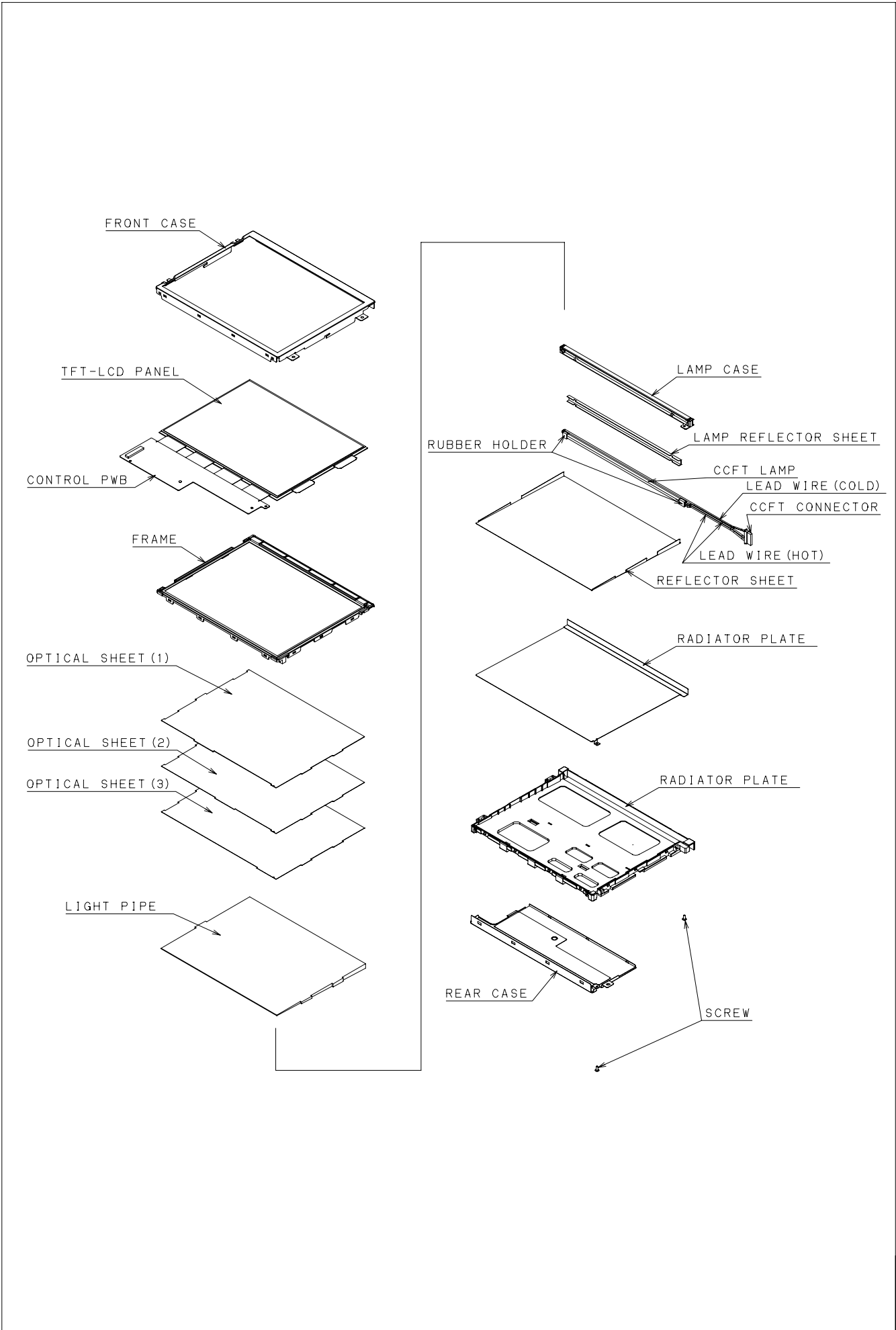
FIG.2 MODULE CONFIGURATION
