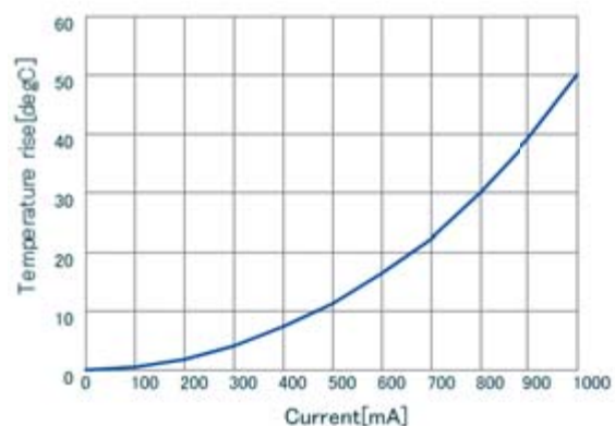
LQM18PN1R5NB0 DT_Current
