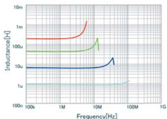
■ LQH43PB6R8M26 L ■ LQH43PB470M26 L ■ LQH43PB221M26 L ■ LQH43PB1R0N26 L
