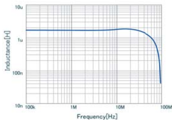
LQM18PN1R5NB0 L
