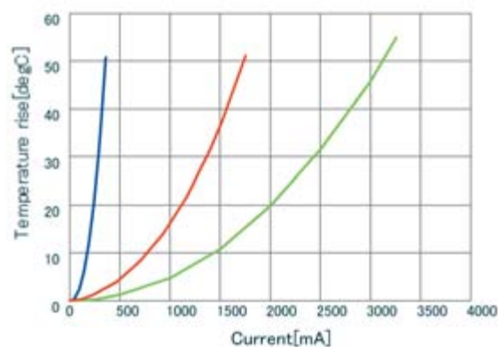
■ LQH43PB221M26 DT_Current ■ LQH43PB2R2M26 DT_Current ■ LQH43PB100M26 DT_Current
