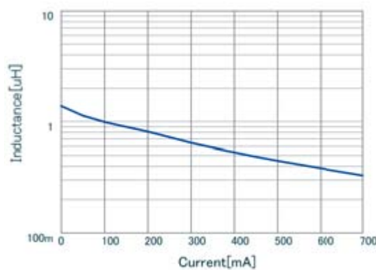
LQM18PN1R5NB0 DC-Bias, 20
