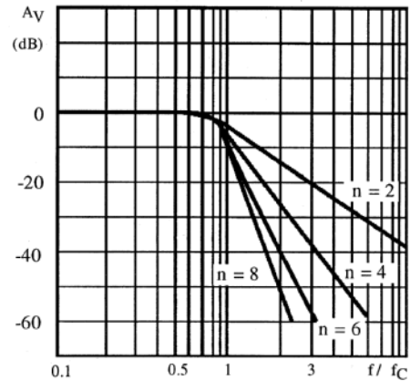
Figure 11. Amplitude response
