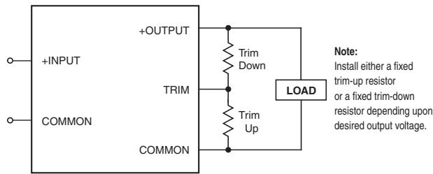
Figure 7. Trim Connections Using Fixed Resistors
