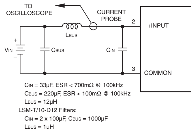
Figure 2. Measuring Input Ripple Current
