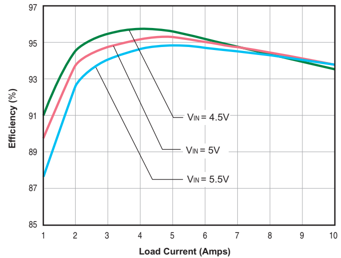
LSM-3.3/10-D5 Efficiency vs. Line Voltage and Load Current
