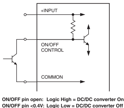
Figure 4. Driving the On/Off Control Pin with an Open-Collector Drive Circuit
