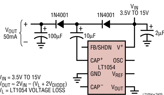
Positive Doubler
